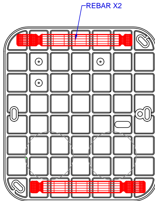
BOTTOM VIEW
