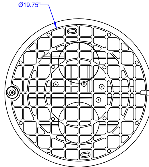
BOTTOM VIEW
